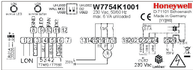
Fig. 6. W7754K sticker with input/output details
