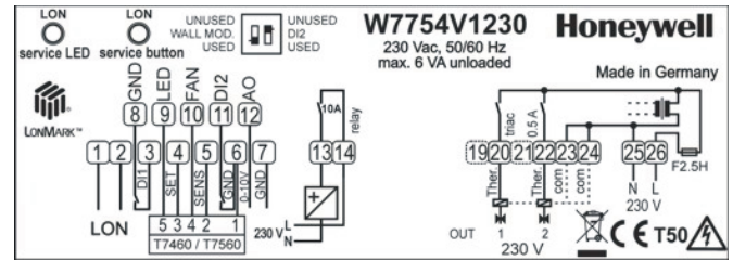
Fig. 11. W7754V sticker with input/output details
