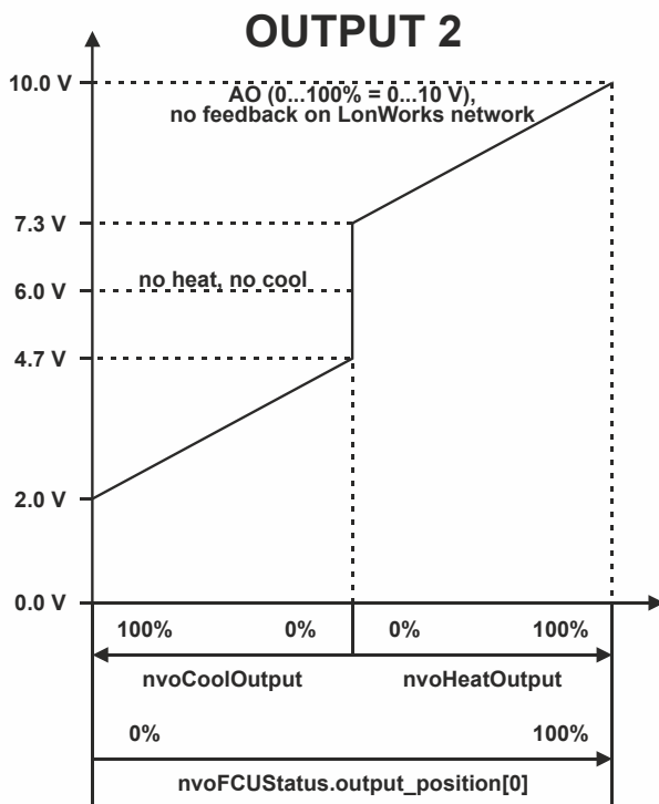
Fig. 4. Operational sequence with Belimo 6-way valve connected to the analog output (2...10 V)
