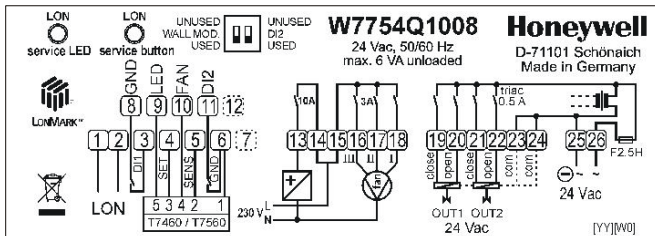
Fig. 8. W7754Q sticker with input/output details
