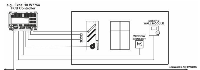
Fig. 5. Typical application
