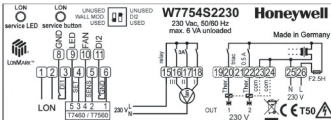
Fig. 10. W7754S sticker with input/output details
