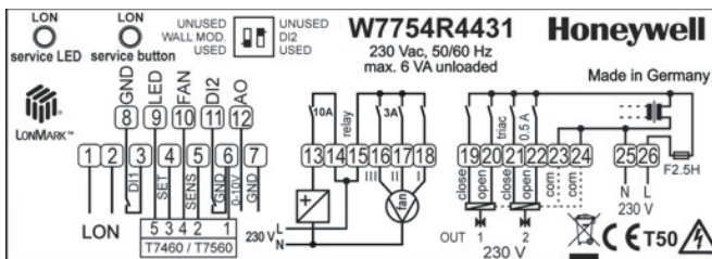
Fig. 9. W7754R sticker with input/output details
