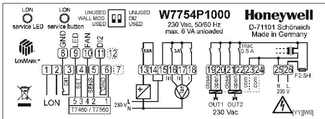
Fig. 7. W7754P sticker with input/output details
