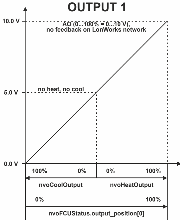
Fig. 3. Operational sequence with “floating mid characteristic” on the analog output (0...10 V)
