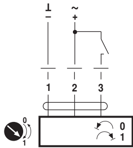
AC/DC 24 V, open-close (one-wire)
