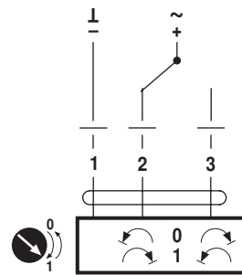
AC/DC 24 V, open-close (two-wire)
